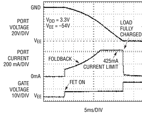
Powering Up into a 180 \mu F Load
