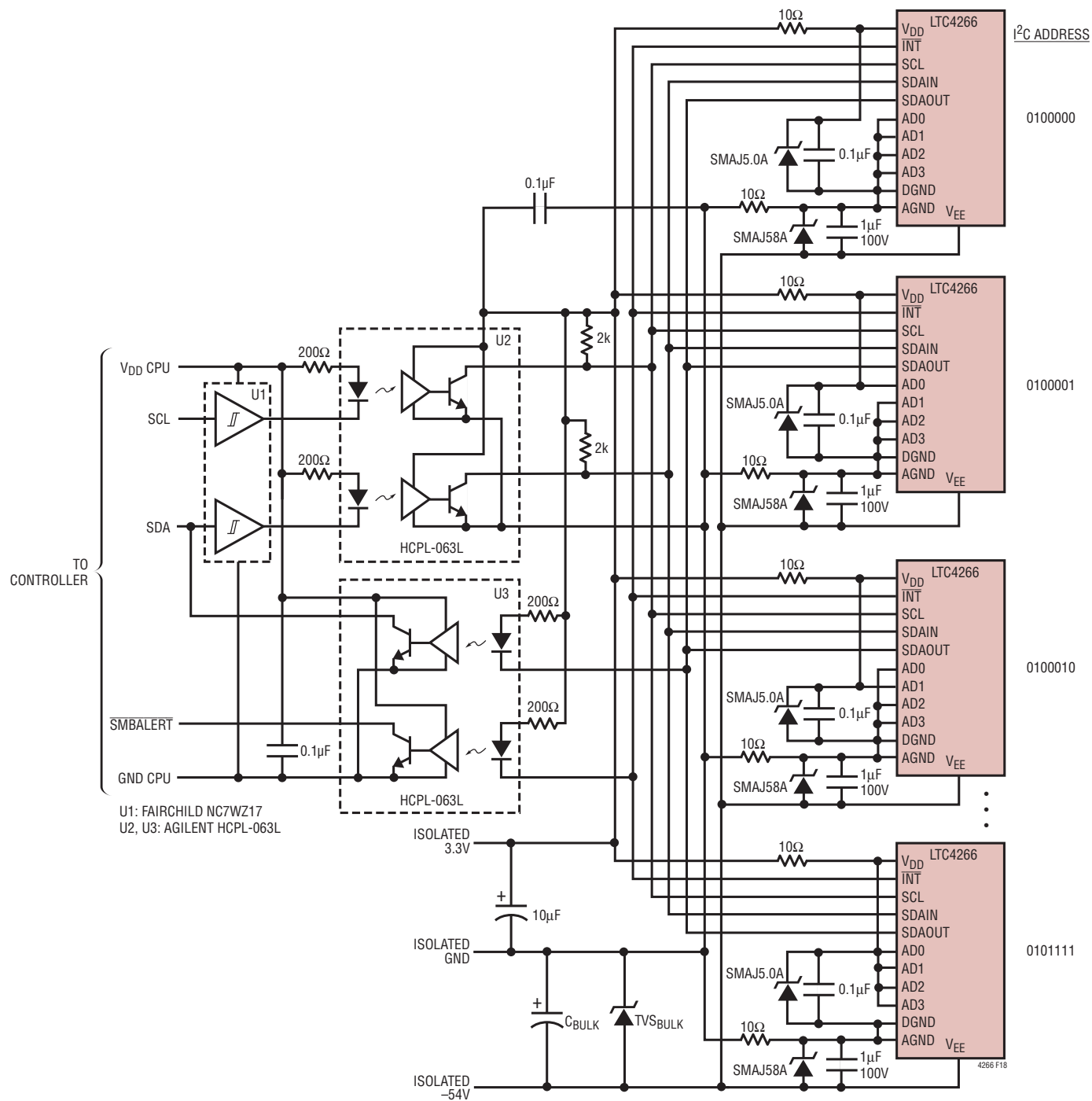
Figure 18. Opto-Isolating the I 2 C Bus
