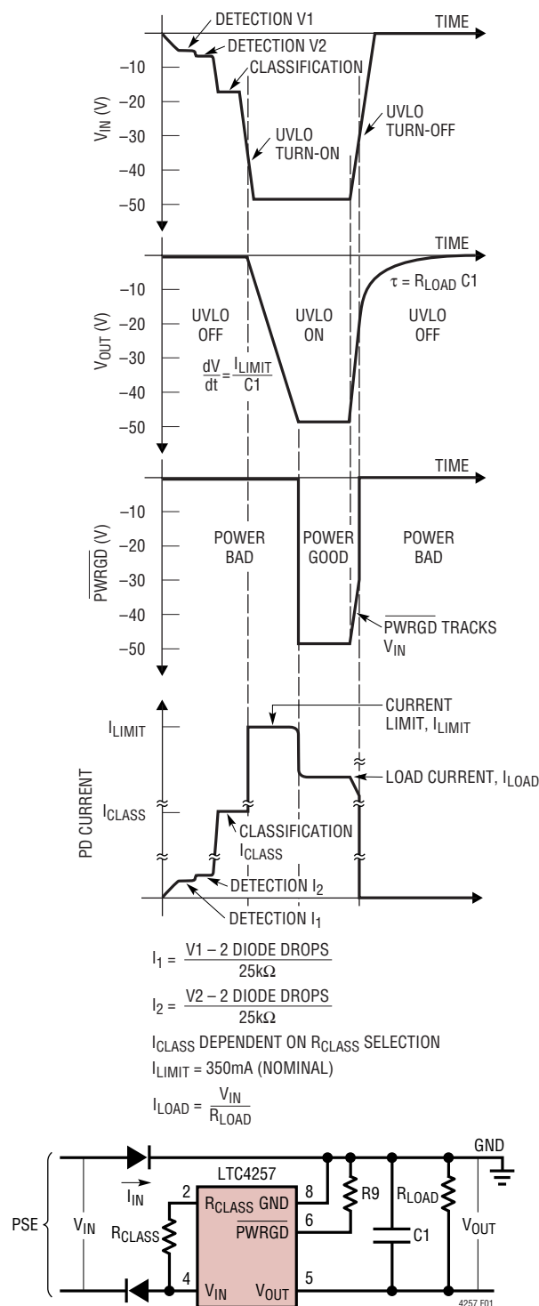
Figure 1. Output Voltage, \overline{\text{PWRGD}} and PD Current as a Function of Input Voltage
