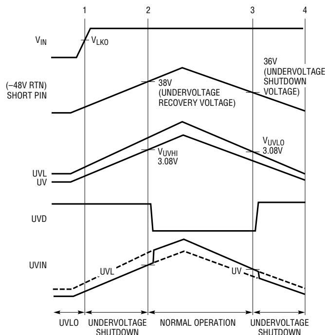
(2a) Undervoltage
