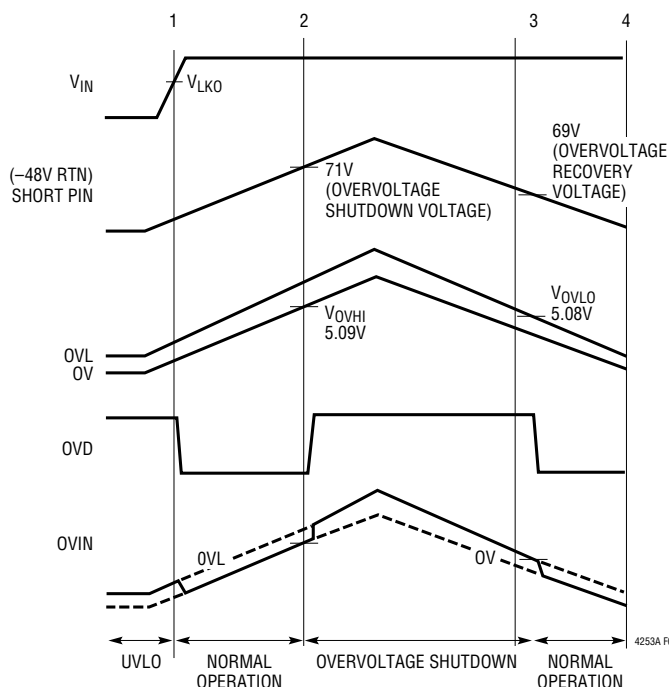
(2b) Overvoltage
