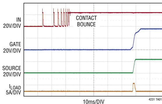
Power-Up Waveforms
