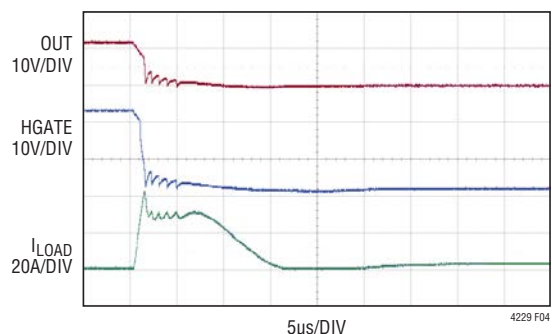
Figure 4. Severe Short-Circuit Fault on 12V Output
