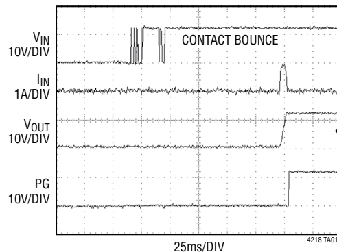
Power-Up Waveform
