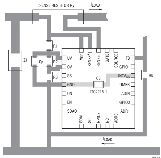
Figure 5. Recommended Layout
