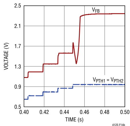
Figure 14. FB, PTH1 and PTH2 Pins Voltage Stepping During a Sweep with C_{TS} = 4.7\text{nF}
