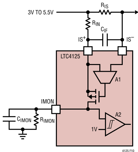
Figure 10. Input Current Limit and Monitoring
