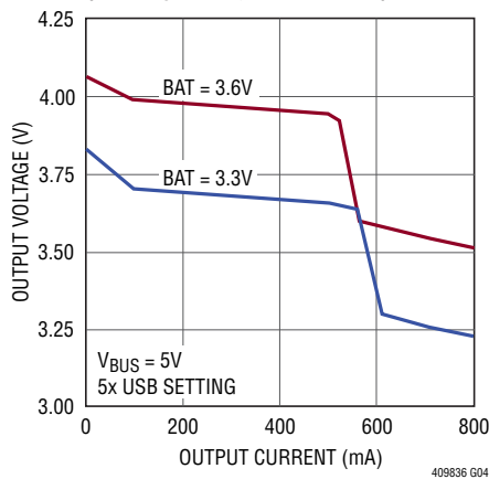
V_{OUT} Voltage vs V_{OUT} Current (Battery Charger Disabled)
