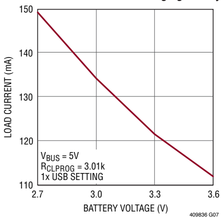
USB Compliant Load Current Available Before Discharging Battery
