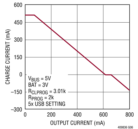
Battery Charge Current vs V_{OUT} Current (Battery Charger Enabled)
