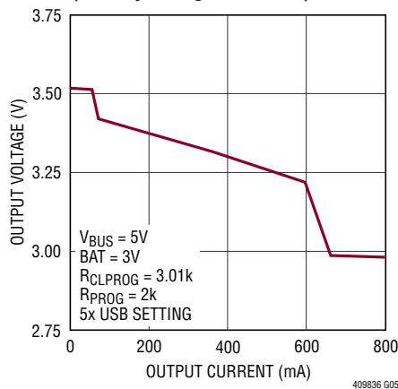
V_{OUT} Voltage vs V_{OUT} Current (Battery Charger Enabled)
