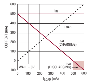
Input and Battery Current vs Load Current R_{\text{PROG}} = 100\text{k} , R_{\text{CLPROG}} = 2\text{k}
