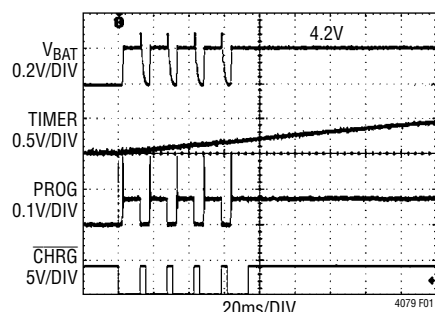
Figure 7. Repeated Charge Terminations on Startup Due to High Resistance of the Battery, C_{\text{TIMER}} = 82\text{nF} , V_{\text{CHG}} = 4.2\text{V} , I_{\text{CHG}} = 10\text{mA} and Battery Resistance = 300\Omega
