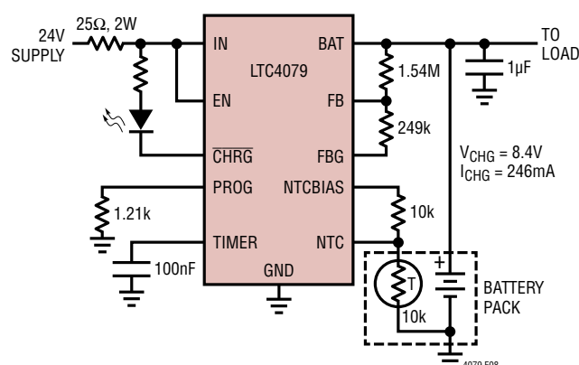
Figure 8. Li-Ion Charger with Timer Termination
