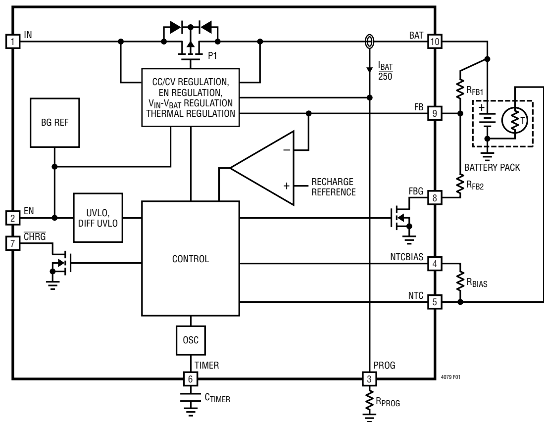
Figure 1. Block Diagram of LTC4079
