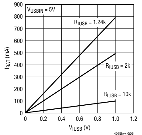
Charge Current vs IUSB Pin Voltage
