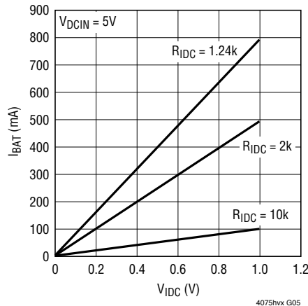
Charge Current vs IDC Pin Voltage
