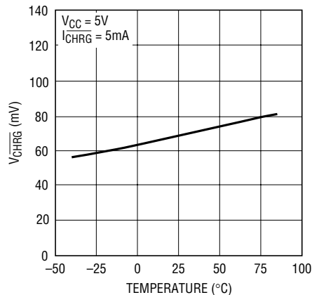
\overline{\text{CHRG}} Pin Output Low Voltage vs Temperature
