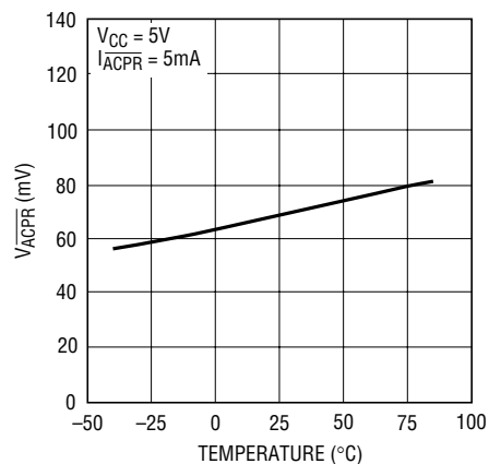
\overline{\text{ACPR}} Pin Output Low Voltage vs Temperature (LTC4065A Only)
