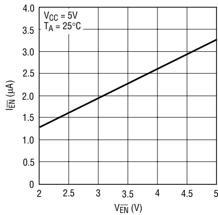
\overline{\text{EN}} Pin Current (LTC4065)
