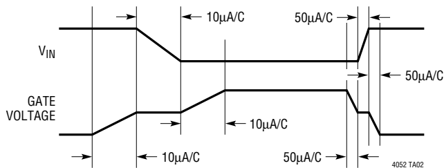
Figure 2. Slew Rate at GATE and V_{\text{IN}} Pins with the RC Network from GATE to V_{\text{IN}}
