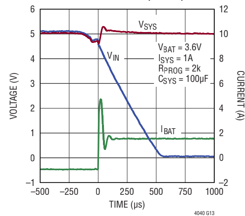
Normal to Backup Mode Transition Waveform (Li-Ion)
