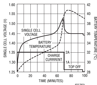
2A NiMH Charge Cycle at 1C
