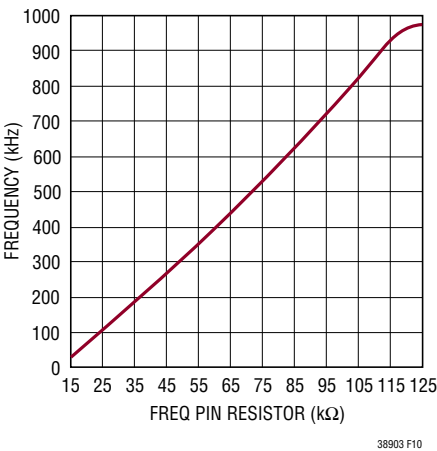
Figure 10. Relationship Between Oscillator Frequency and Resistor Value at the FREQ Pin
