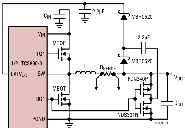
Figure 9. Capacitive Charge Pump for EXT V CC
