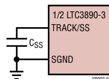
Figure 6. Using the TRACK/SS Pin to Program Soft-Start
