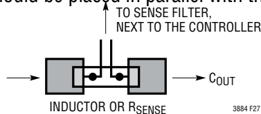
Figure 27. Sense Lines Placement with Inductor DCR
