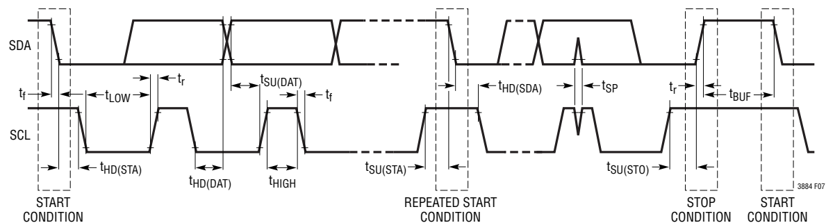
Figure 7. Timing Diagram
