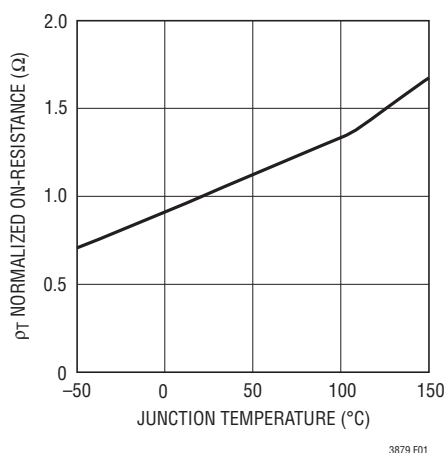
Figure 1. R_{DS(ON)} vs Temperature
