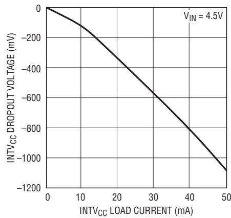
INTV_{CC} Dropout
