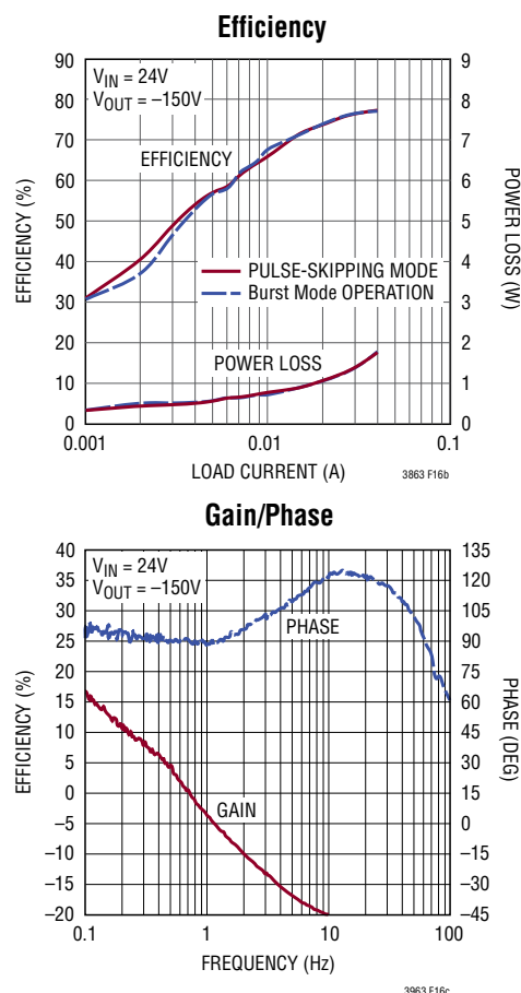
Gain/Phase Measurements Taken with OMICRON Lab Bode 100 Vector Network Analyzer.
