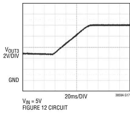
Soft Start-Up (Boost)
