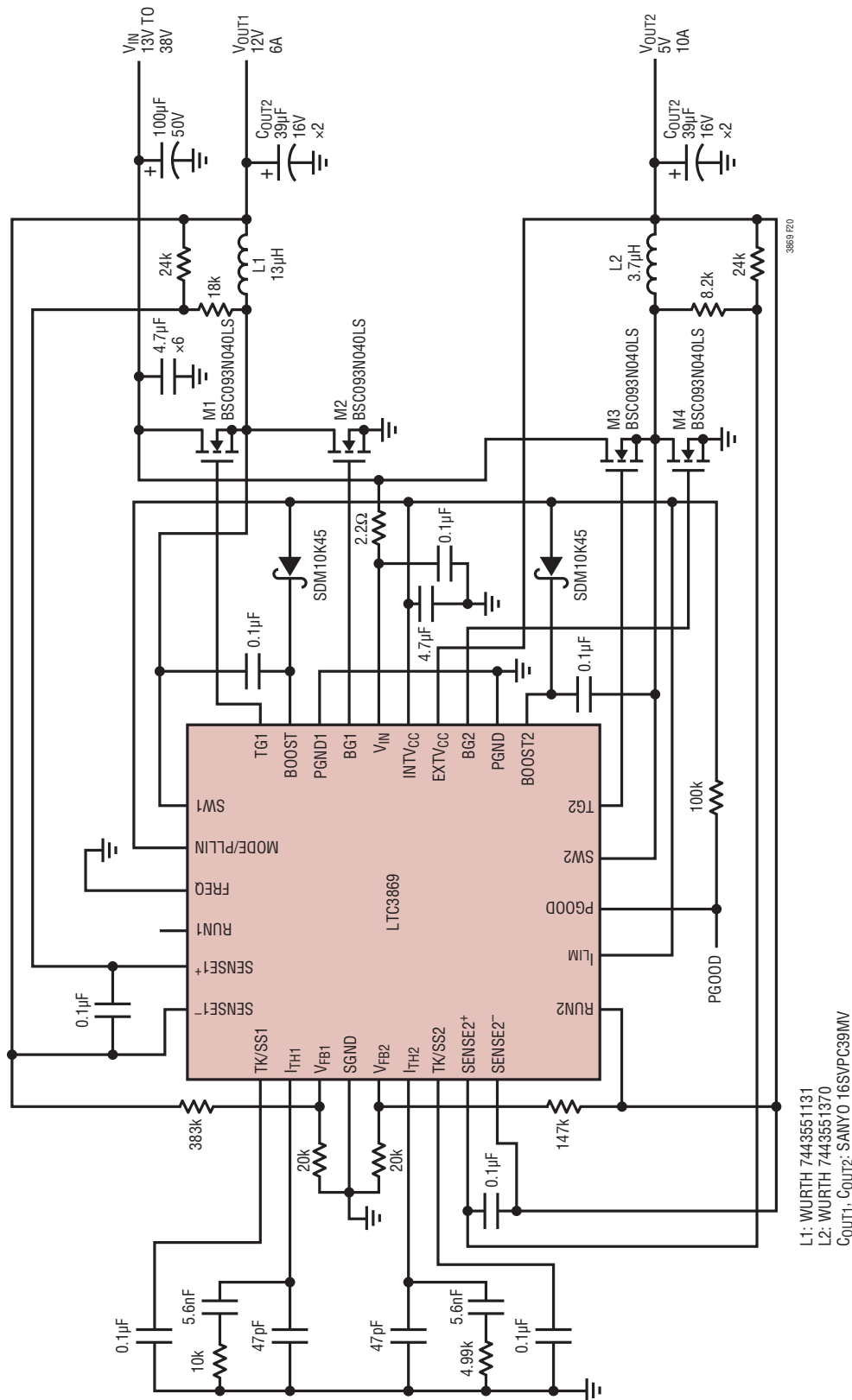
Figure 20. 12V, 6A and 5V, 10A Supply with DCR Sensing, f_{sw} = 250\text{kHz}
