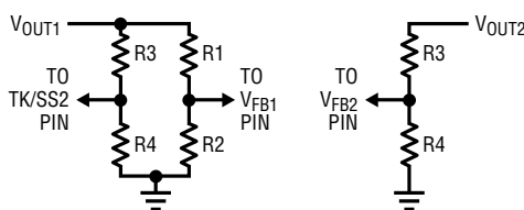
(12a) Coincident Tracking Setup
