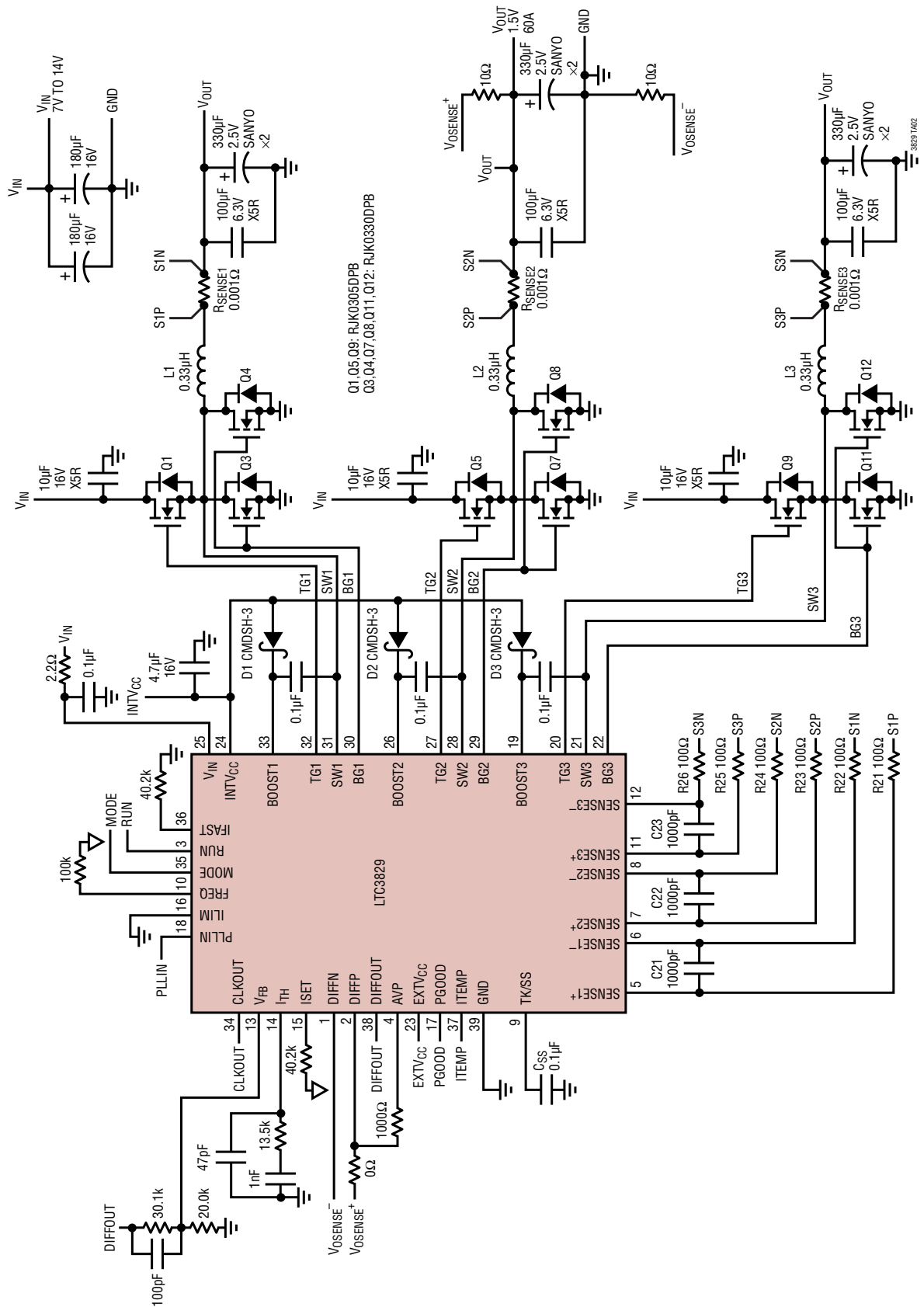
1.5V, 60A Converter Using Sense Resistors, f_{sw} = 400\text{kHz}
