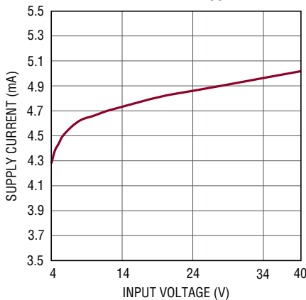
Quiescent Current vs Input Voltage without EXTV_{CC}
