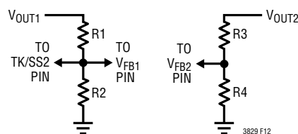
(12b) Ratiometric Tracking Setup
