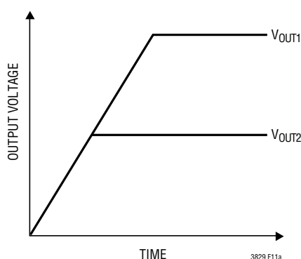
(11a) Coincident Tracking
