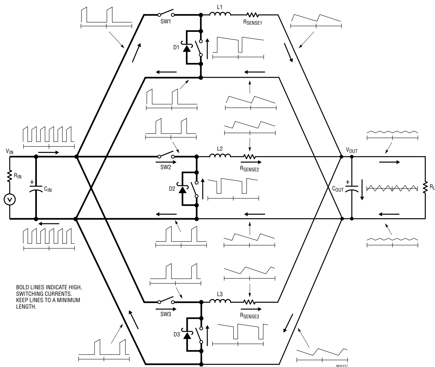
Figure 17. Branch Current Waveform
