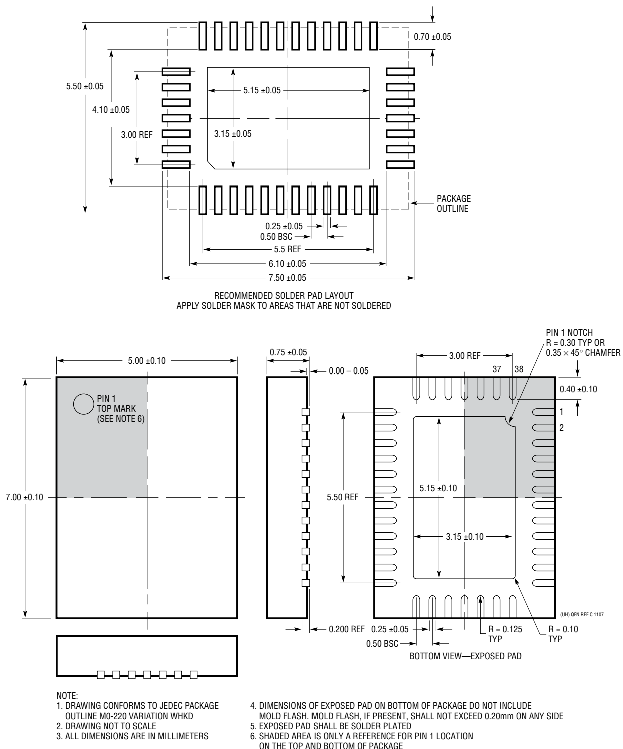
UHF Package 38-Lead Plastic QFN (5mm × 7mm) (Reference LTC DWG # 05-08-1701 Rev C)
