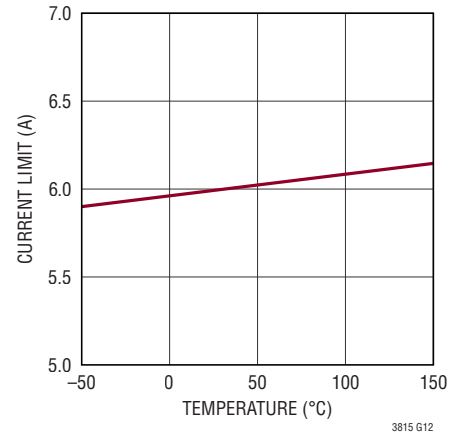
Valley Current Limit vs Temperature
