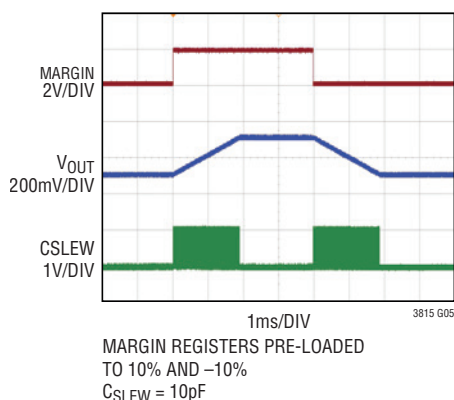
Output Margining
