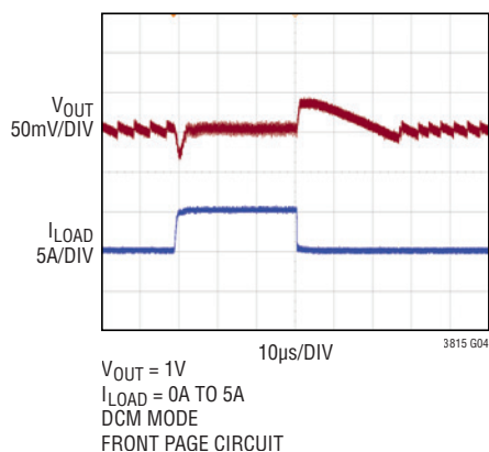
Load Step (Discontinuous Mode)
