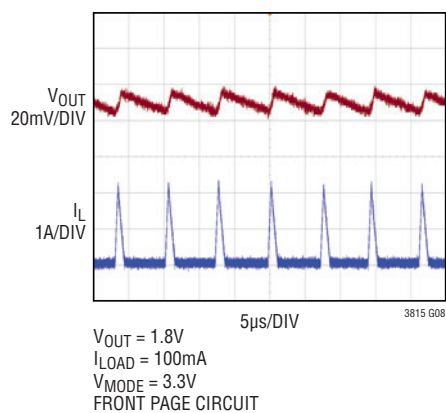
Discontinuous Mode Operation
