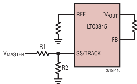
Figure 13c. Slave IC Circuit for Coincident Tracking and V_{MASTER} \geq V_{SLAVE}
