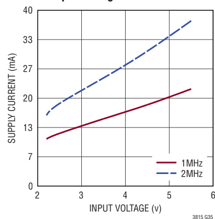
Dynamic Supply Current vs Input Voltage
