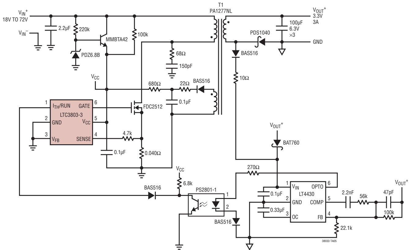
4:1 Input Range 3.3V Output Isolated Flyback DC/DC Converter
