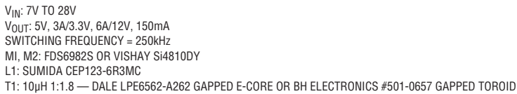
Figure 12. LTC3728L-1 High Efficiency Low Noise 5V/3A, 3.3V/5A, 12V/120mA Regulator
