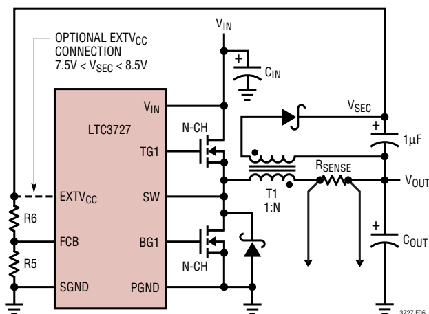
Figure 6. Secondary Output Loop &amp; EXTVCC Connection
