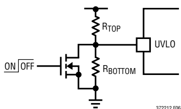
Figure 6. System UVLO Setup
