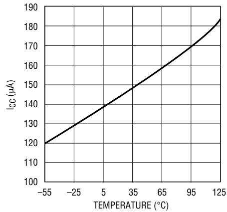
Start-Up I_{CC} vs Temperature
