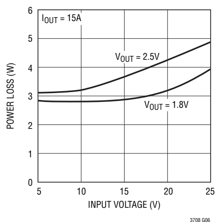
Power Loss vs Input Voltage
