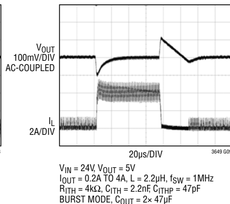
Transient Response, Burst Mode
