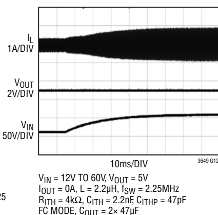
Output Regulation with V_{IN} Slew
