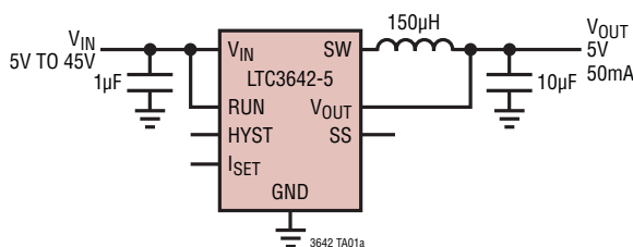
5V, 50mA Step-Down Converter
