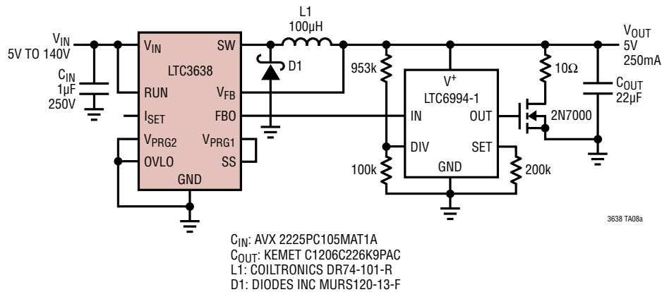
5V to 140V Input to 5V/250mA Output with 20kHz Minimum Burst Frequency
