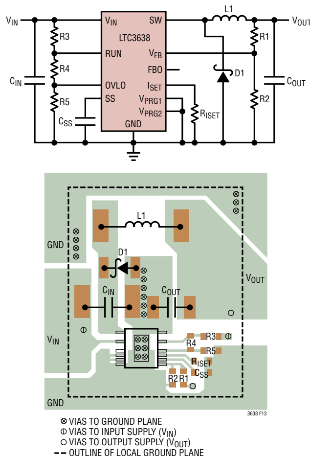
Figure 13. Example PCB Layout
