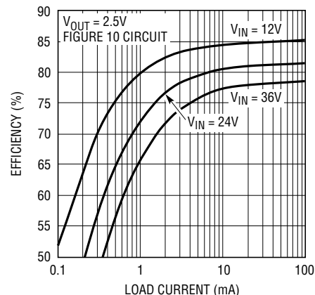
Efficiency vs Load Current, V_{OUT} = 2.5V
