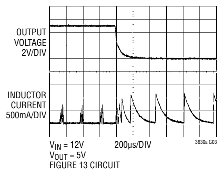
Short-Circuit Response
