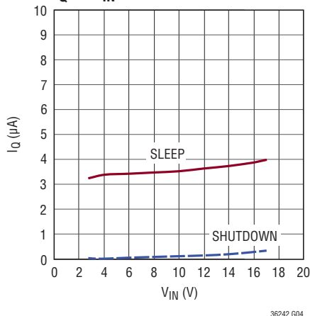
I_Q vs V_{IN}
