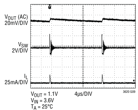
Switching Waveforms at 250μA Load, FMIN/MODE = 0V
