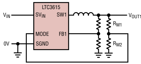
2b. Burst Mode Operation Externally Controlled
