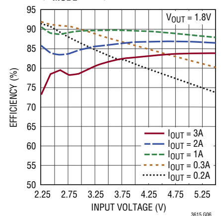
Efficiency vs Input Voltage (V_{MODE} = 0V)
