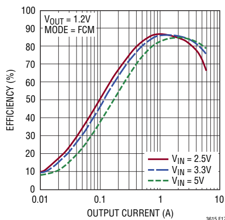
Figure 17. Efficiency vs Load Current for V_{OUT} = 1.2V and I_{OUT} Up to 6A
