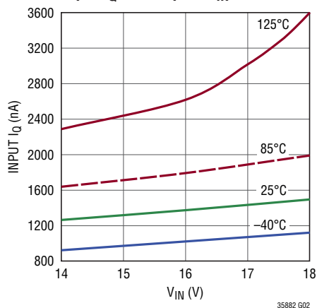
Input I_Q in Sleep vs V_{IN}
