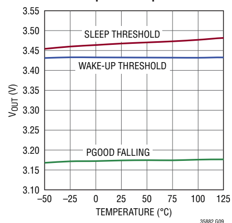
3.45V Output vs Temperature
