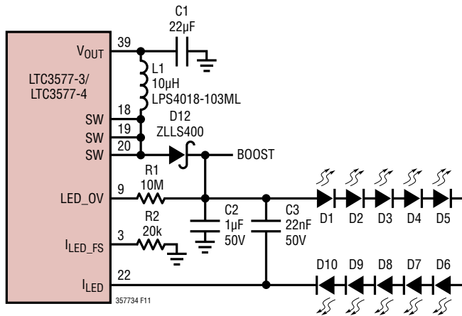
Figure 11. LED Boost Application Circuit
