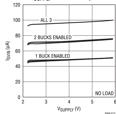
I_{\text{SVIN}} vs V_{\text{SUPPLY}} Burst Mode Operation
