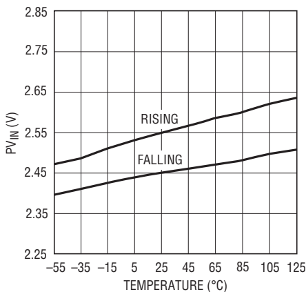
Buck Regulator \text{PV}_{\text{IN}} Undervoltage Thresholds vs Temperature
