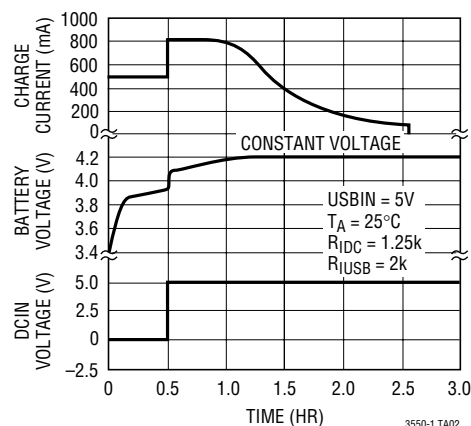
Complete Charge Cycle (1100mA Battery)
