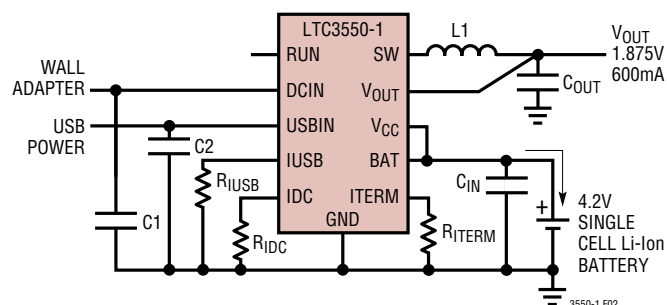
Figure 2. LTC3550-1 Basic Circuit
