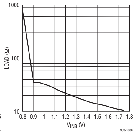
Minimum Load Resistance During Start-Up vs V_{\text{INB}}
