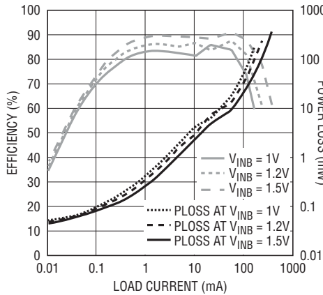
Efficiency vs Load Current and V_{\text{INB}} for V_{\text{OUTB}} = 1.8\text{V}
