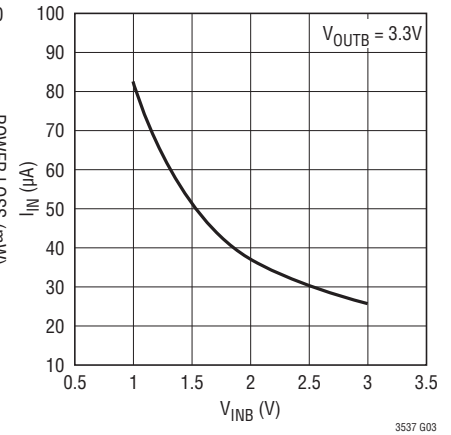
No-Load Input Current vs V_{\text{INB}}
