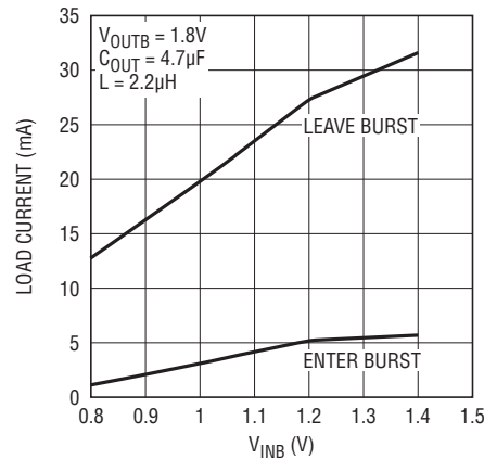
Burst Mode Threshold Current vs V_{\text{INB}}
