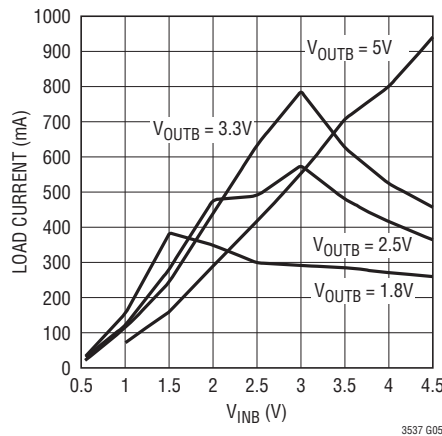
Maximum Output Current vs V_{\text{INB}}
