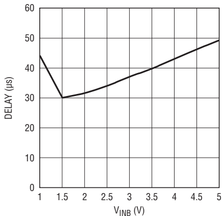
Start-Up Delay Time vs V_{\text{INB}}
