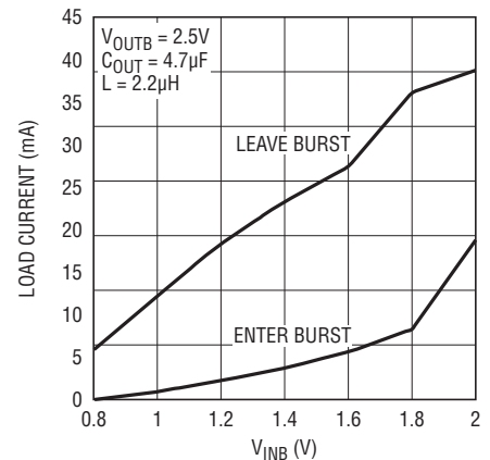
Burst Mode Threshold Current vs V_{\text{INB}}
