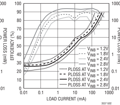
Efficiency vs Load Current and V_{\text{INB}} for V_{\text{OUTB}} = 3.3\text{V}
