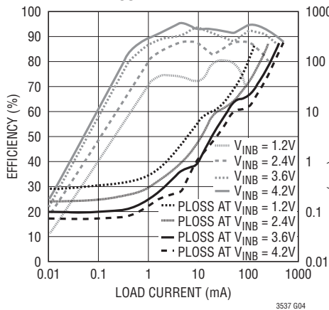
Efficiency vs Load Current and V_{\text{INB}} for V_{\text{OUTB}} = 5\text{V}
