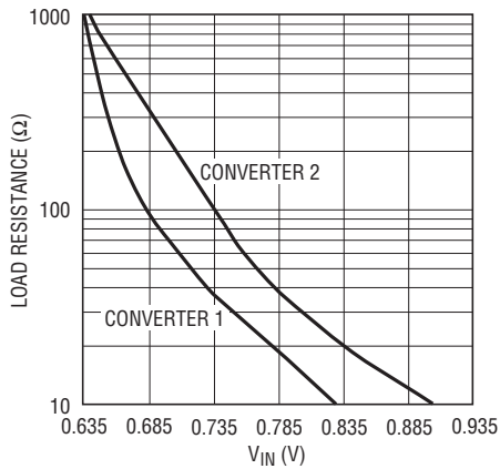
Minimum Load Resistance During Start-Up vs V IN
