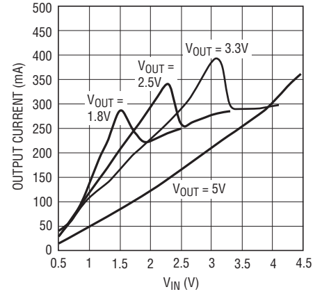
Maximum Output Current vs V IN for Converter 2
