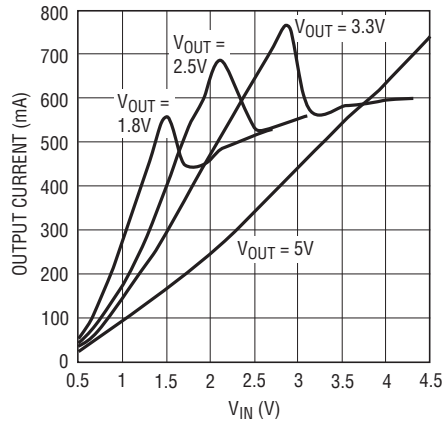
Maximum Output Current vs V IN for Converter 1
