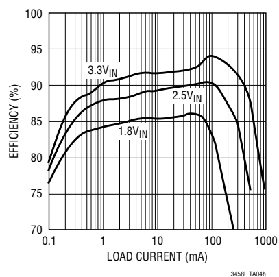
Two Alkaline to 5V OUT
