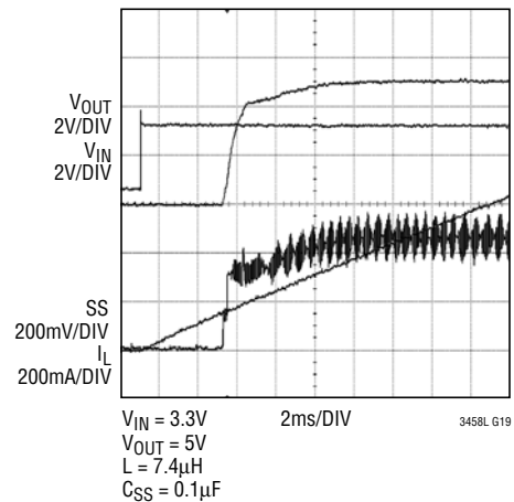
Soft-Start into 20\Omega Load
