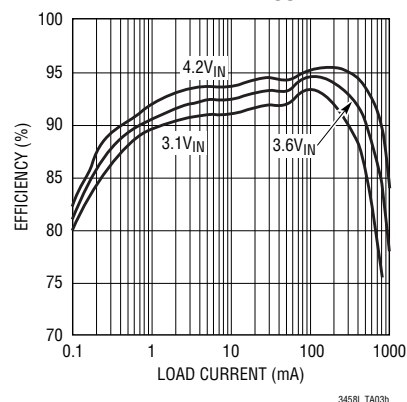
Li-Ion to 5V OUT
