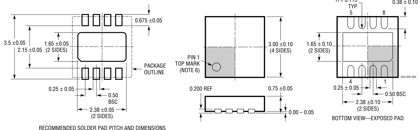
DD Package 8-Lead Plastic DFN (3mm × 3mm) (Reference LTC DWG # 05-08-1698)
