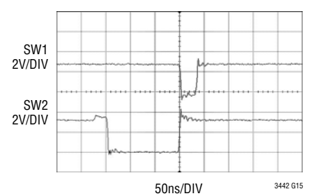
Switch Pins Before Entering Boost Mode
